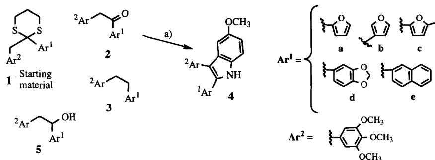
Figure 2. Synthesis of 1-3 and 5 according to Refs. 12, 13, 14; a ) p\text{-CH}_3\text{O-C}_6\text{H}_4\text{-NH-NH}_2 , AcOH, EtOH, 1.5 h, reflux
