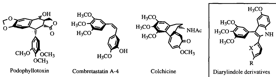
Figure 1. Representative examples of antineoplastic bridged biaryls.
